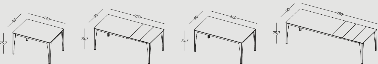
Tavolo allungabile con struttura e gambe in metallo verniciato e piano in laminato sp. 2 cm. Extendable table with metal painted structure and legs, and 2 cm thick laminate top.
