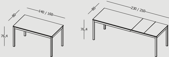
Tavolo allungabile con struttura e gambe in alluminio verniciato con piano in laminato sp. 2 cm. Extendable table with painted aluminium structure and legs, and 2 cm thick laminate top.
