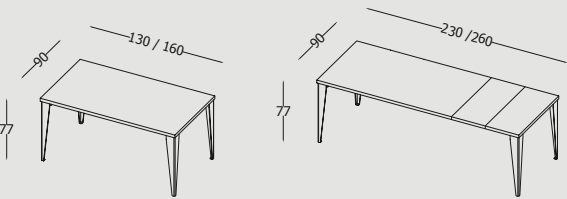
Tavolo allungabile con struttura e gambe in metallo verniciato e piano in laminato sp. 2 cm. Extendable table with metal painted structure and legs, and 2 cm thick laminate top.
