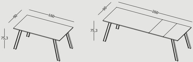
Tavolo allungabile con gambe in metallo verniciato e piano in laminato sp. 2 cm. Extendable table with painted metal legs and 2 cm thick laminate top.
