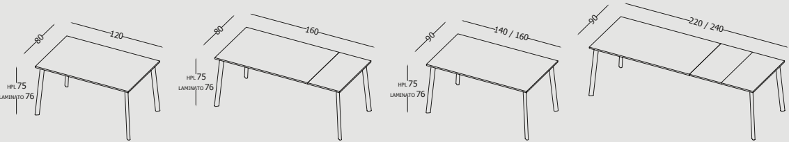
Tavolo allungabile con struttura in acciaio, gambe in alluminio verniciato e piano in laminato sp. 2 cm o HPL sp. 1 cm. Extendable table with steel structure, painted aluminium legs and 2 cm thick laminate or 1 cm thick HPL top.
