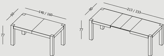
Tavolo allungabile interamente in laminato con lavorazione folding. Extendable table made entirely in laminate, with folding system.
