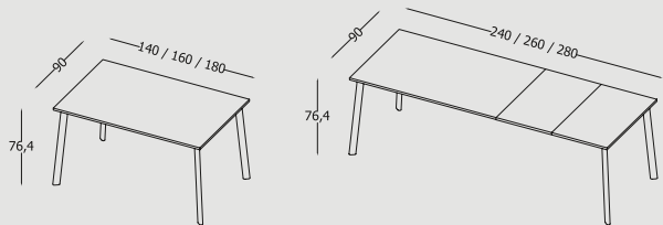
Tavolo allungabile con piano sp. 2 cm in laminato e gambe in metallo verniciato. Extendable table with 2 cm thick laminate top and painted metal legs.
