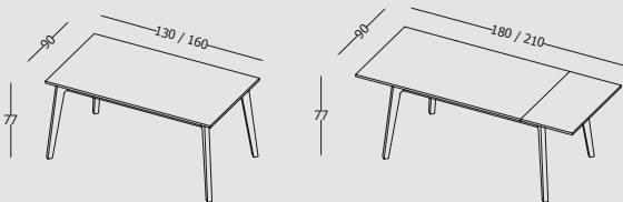
Tavolo allungabile con struttura e gambe in legno verniciato e piano in laminato sp. 2 cm. Extendable table with painted wood structure and legs, and 2 cm thick laminate top.
