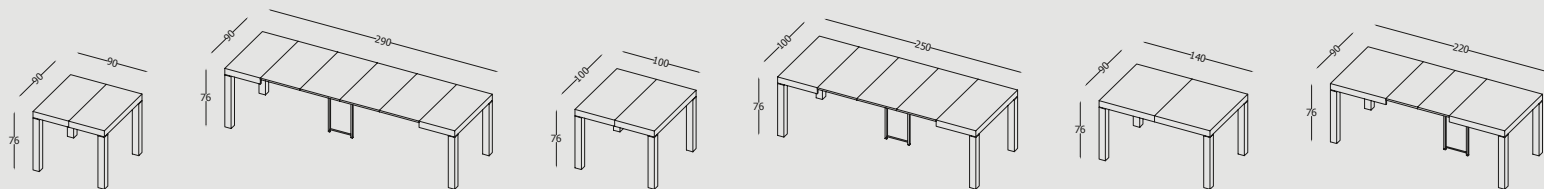
Tavolo allungabile telescopico con gambe in metallo verniciato e piano in melaminico con lavorazione folding. Telescopic extendable table with painted metal legs and melamine top with folding system.
