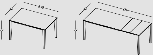
Tavolo allungabile con struttura e gambe in metallo verniciato e piano in laminato sp. 2 cm. Extendable table with metal painted structure and legs, and 2 cm thick laminate top.
