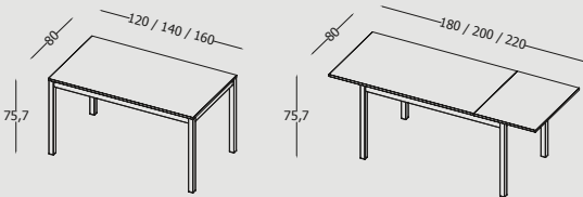
Tavolo allungabile con struttura e gambe in metallo verniciato e piano in laminato sp. 2 cm. Extendable table with metal painted structure and legs, and 2 cm thick laminate top.
