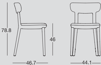
Sedia con monoscocca in polipropilene, seduta imbottita e rivestita in tessuto. Chair with polypropylene monobloc and padded seat upholstered in fabric.
