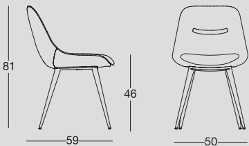
Sedia con struttura in metallo verniciato nero e seduta rivestita in eco-nabuk. Chair with black painted metal structure and seat upholstered in eco-nabuk.
