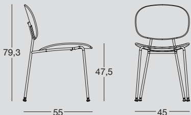
Sedia con struttura in acciaio verniciato o cromato, seduta e schienale in polipropilene. Chair with painted steel or chrome-plated structure, and polypropylene seat and back.
