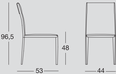
Sedia con struttura in metallo, imbottita e completamente rivestita in ecopelle. Chair with metal structure, padded and entirely upholstered in eco-leather.
