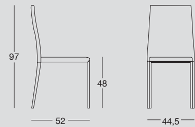
Sedia con struttura in metallo completamente rivestita in ecopelle. Chair with metal structure, entirely upholstered in eco-leather.
