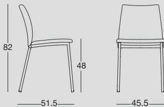
Sedia con struttura in metallo verniciato e seduta imbottita rivestita in ecopelle. Chair with painted metal structure and padded seat upholstered in eco-leather.
