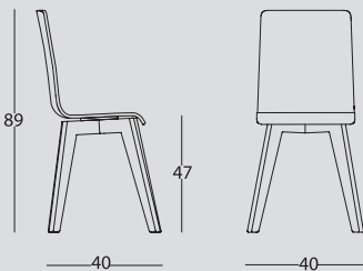
Sedia con struttura in legno e seduta in multistrato rivestito in Fenix. Chair with wood structure and plywood seat coated with Fenix.
