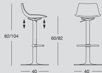
Sgabello con basamento regolabile tramite pistone a gas con seduta in polipropilene con cuscinetto rivestito in ecopelle. Stool and base with gas-lift adjustment, and polypropylene seat with cushion upholstered in eco-leather.
