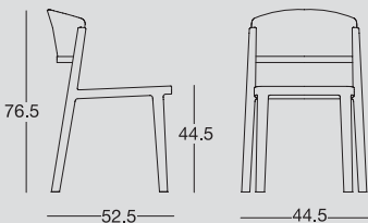
Sedia bi-materiale in tecnopolimero. Chair made of techno-polymer twin-material.
