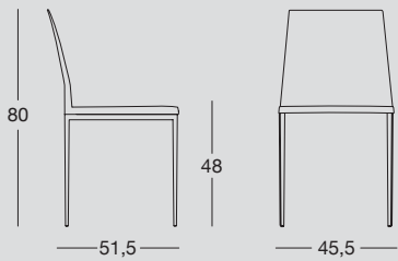
Sedia con struttura in metallo verniciato o cromato e seduta in polipropilene. Chair with painted or chrome-plated metal structure and polypropylene seat.
