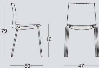
Sedia con gambe in metallo verniciato e scocca in tecnopolimero. Chair with painted metal legs and technopolymer shell.
