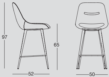
Sgabello con struttura in metallo verniciato nero e seduta rivestita in eco-nabuk. Stool with black painted metal structure and seat upholstered in eco-nabuk.
