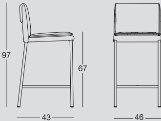
Sgabello con struttura in metallo, seduta imbottita completamente rivestita in ecopelle con poggiatesta in metallo verniciato nero. Stool with metal structure, padded and entirely upholstered eco-leather seat, with black painted metal footrest.
