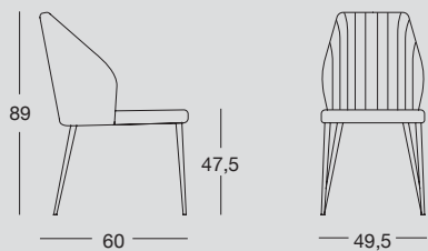
Sedia con struttura in metallo, imbottita e completamente rivestita in ecopelle. Chair with metal structure, padded and entirely upholstered in eco-leather.
