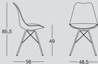
Sedia con struttura in metallo verniciato, seduta in polipropilene con cuscino in ecopelle. Chair with painted metal structure, polypropylene seat and eco-leather cushion.
