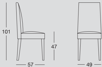
Sedia con struttura in legno laccato e seduta imbottita e rivestita in ecopelle. Chair with lacquered wood structure and padded seat upholstered in eco-leather.
