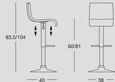
Sgabello con basamento regolabile tramite pistone a gas con seduta rivestita in ecopelle. Stool and base with gas-lift adjustment, and seat upholstered in eco-leather.
