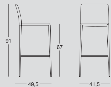
Sgabello con struttura in metallo verniciato, seduta e schienale imbottiti e rivestiti in ecopelle vintage. Stool with painted metal structure, padded seat and back upholstered in vintage eco-leather.
