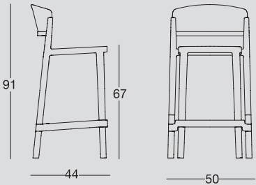
Sgabello bi-materiale in tecnopolimero. Chair made of techno-polymer twin-material.
